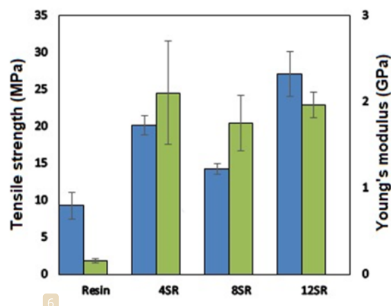
Fig. 8. Tensile strength and the Young's modulus of neat epoxy adhesive resin, and composites based on cellulose fibers fabricated from oil palm empty fruit bunch fibers subjected to 4, 8, and 12 pretreatment cycles with a 4 wt% aqueous solution of NaOH followed by blending (4SR, 8SR, and 12SR, respectively).
