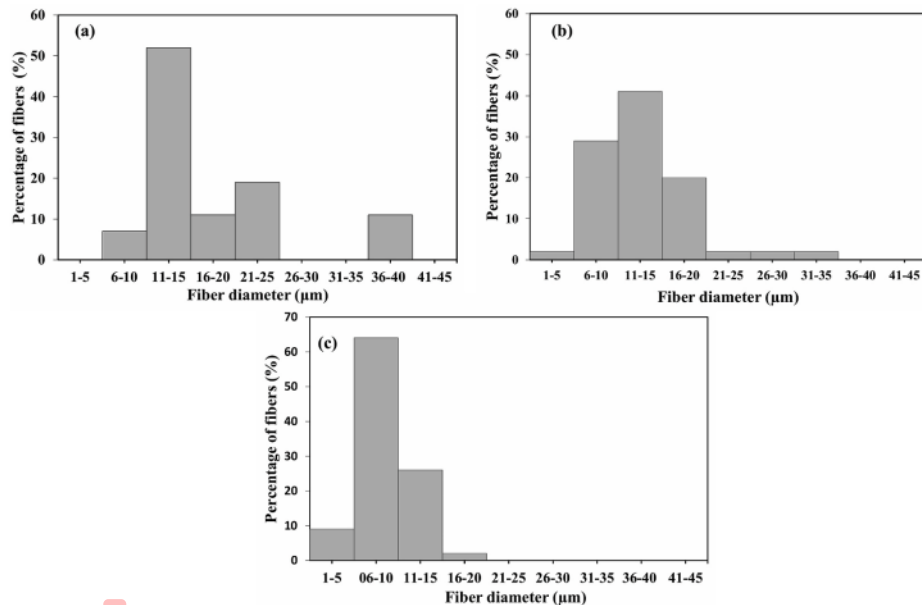
Fig. 3. Diameter distribution of cellulose fibers fabricated from oil palm empty fruit bunch fibers subjected to (a) 4, (b) 8, and (c) 12 pretreatment cycles with a 4 wt% aqueous solution of NaOH followed by blending.
