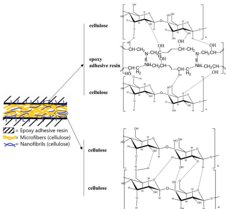
Fig. 11. Schematic diagram of possible interactions between the epoxy adhesive resin, cellulose microfibrils, and cellulose nanofibrils.
