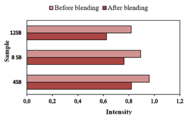
Fig. 6. The intensities of Fourier-transform infrared spectra peaks of lignin (1639 cm -1 ) comparison between before and after blending in different pretreatments.
